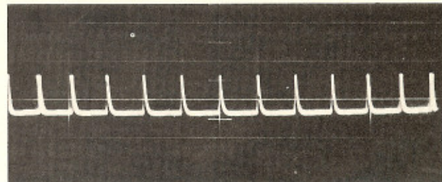
1 kilocycle trigger output of the Type 180 displayed on a TEKTRONIX Type 513-D Oscilloscope.
