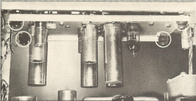
SHOCK MOUNTING OF TYPE 121 PRE-AMPLIFIER
