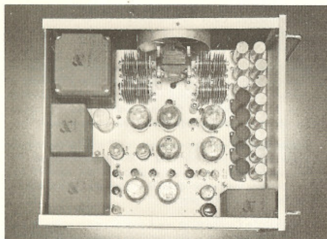
POWER SUPPLY
